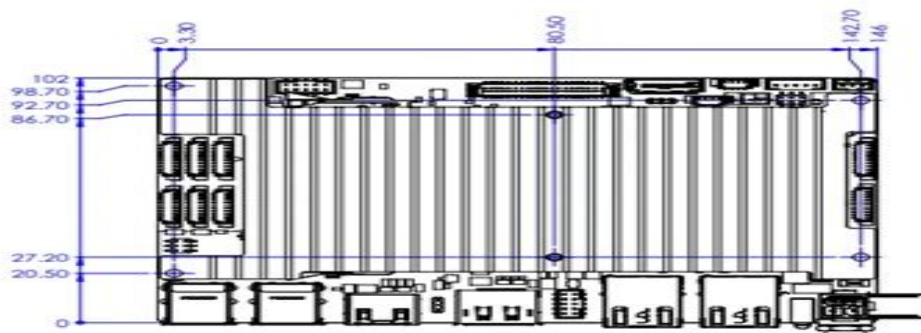
Figure 4. Mechanical Diagram with Heatsink (Top Side)
