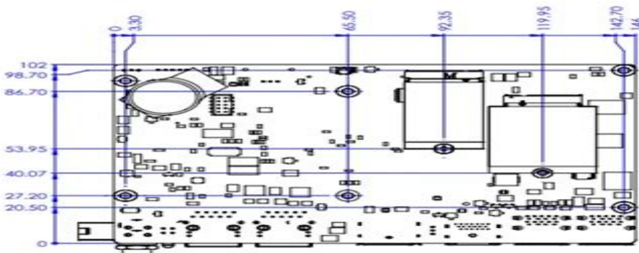
Figure 5. Mechanical Diagram with Heatsink (Bottom Side)
