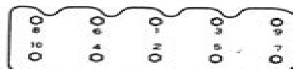
Cylinder head bolt tightening sequence
