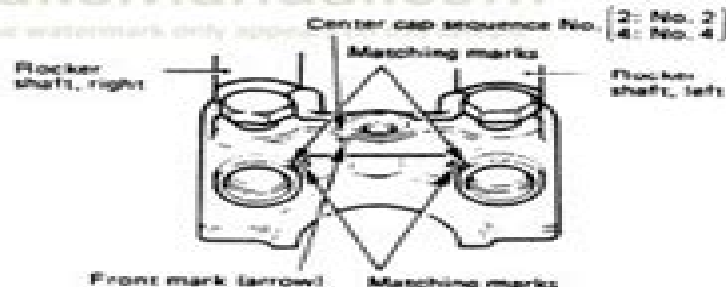
Matching marks for positioning rocker shafts
