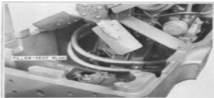
Figure A2-24 Manual Steering Gear Filler-Test Plug
