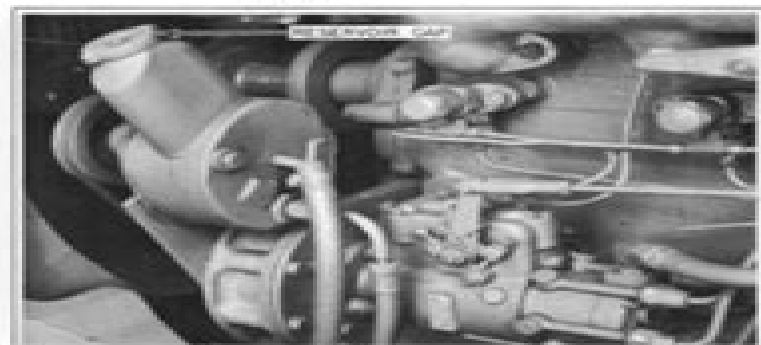
Figure A2-25 Power Steering Pump
