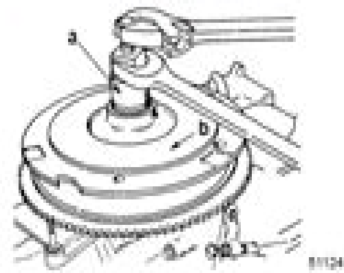
a - Flywheel Holder
