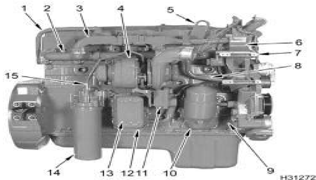
Figure 8 Component location – right
