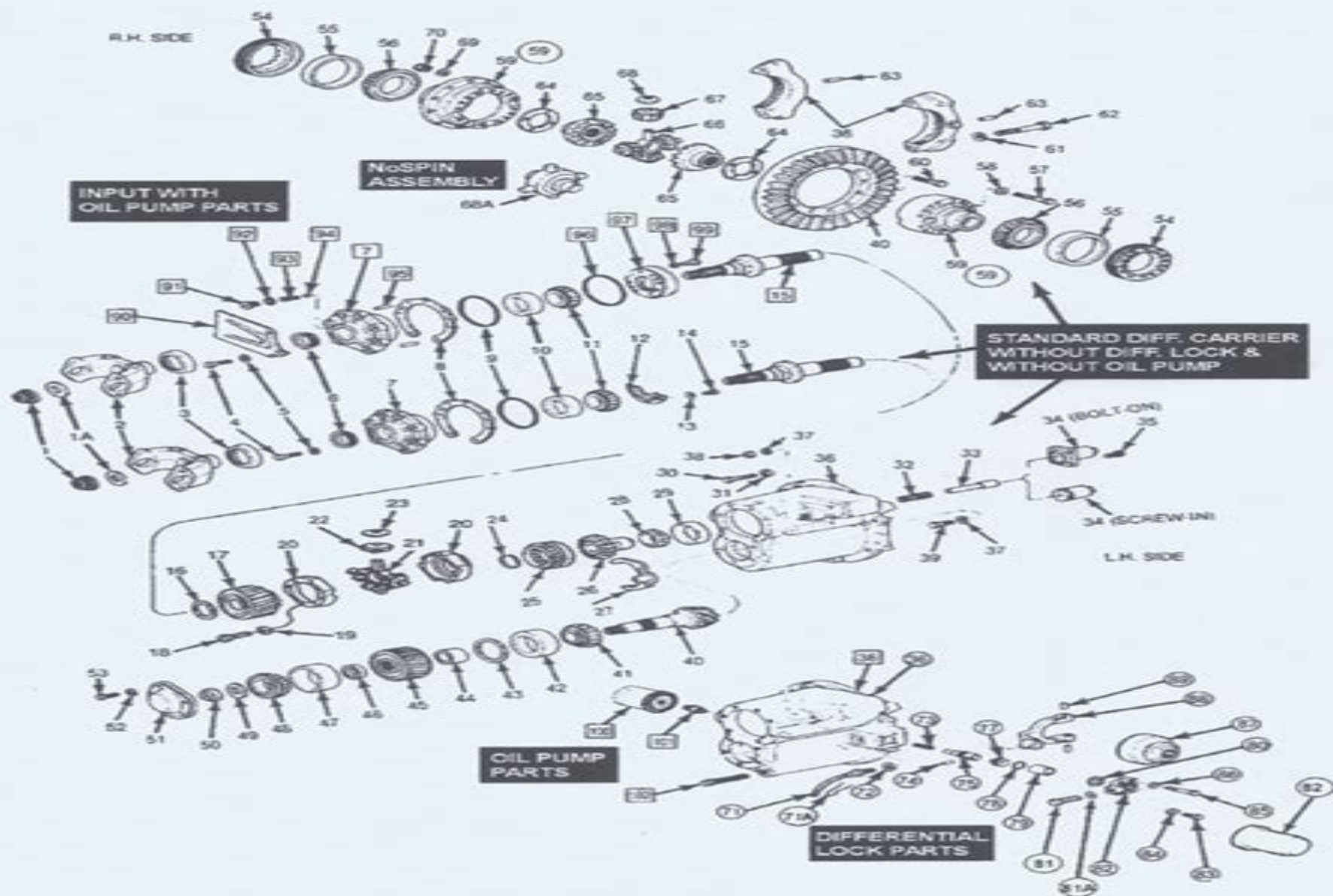
FIGURE 1 FORWARD CARRIERS OF TANDEM AXLES (USE WITH CHART 1)
