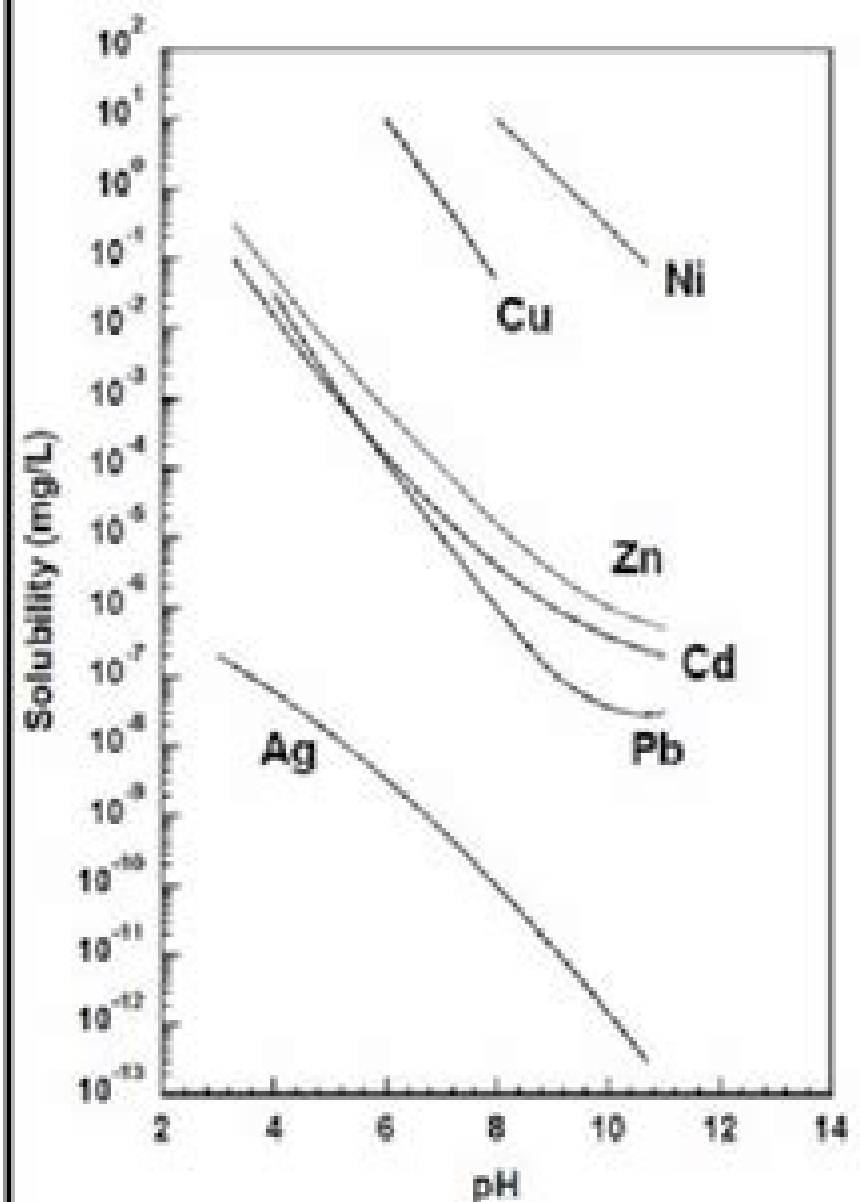
Metal sulphide
