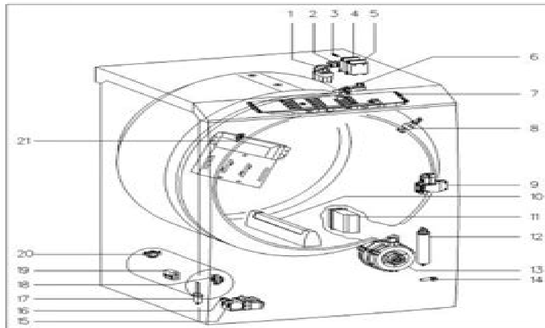
Figure D-2: T 982x Component Layout
