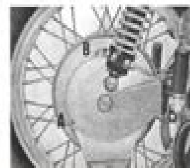
Rear wheel drive oil level, filter, and drain plugs (V750 and V750i)
