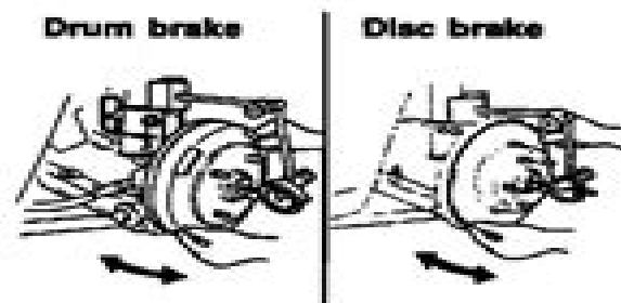
Fig. 1 Checking Wheel Bearing Endplay
