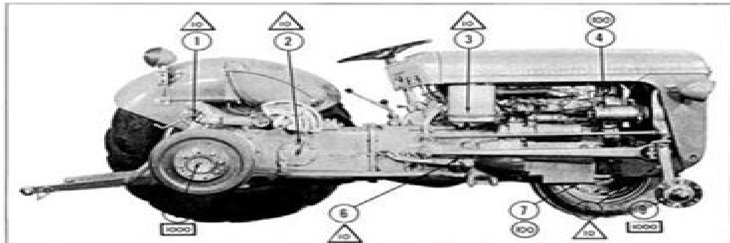
Lubrication Chart
