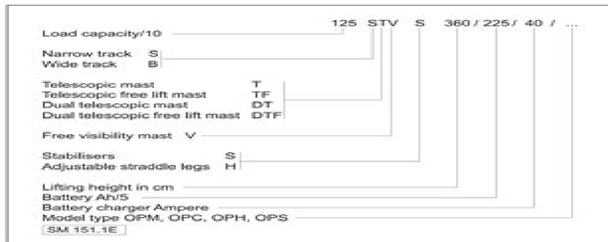
Figure 1.2 Type designations (example)
