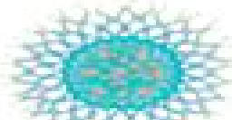
AgNPs
