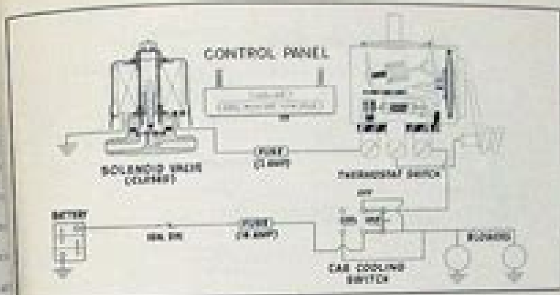
Fig. 8b Schematic Wiring Diagram of Control Circuit
