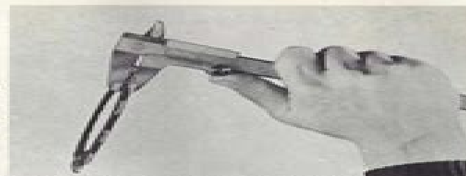
Fig. 7-12-8 Measuring cork plate thickness
