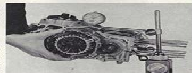
Fig. 7-12-10 Measuring backlash with dial gauge
