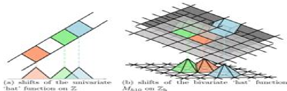
Figure 1: Box splines as a projection of n -dimensional boxes [38].
