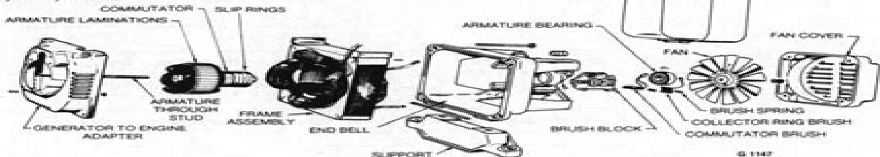
FIGURE 41. TYPICAL GENERATOR PARTS BREAKDOWN
