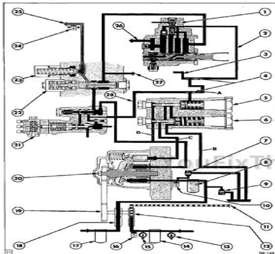
Control of Variable Displacement Piston Pump with Top Link Sending Hydraulic Lift Assembly Unload Valve (Fast Lift)
