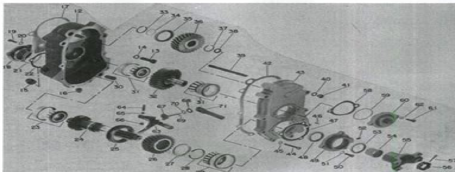
Fig. 19—Exploded view of the four-wheel drive transfer drive assembly. Breather filter element (not shown) should be renewed yearly, or after each 1000 hours of operation.
