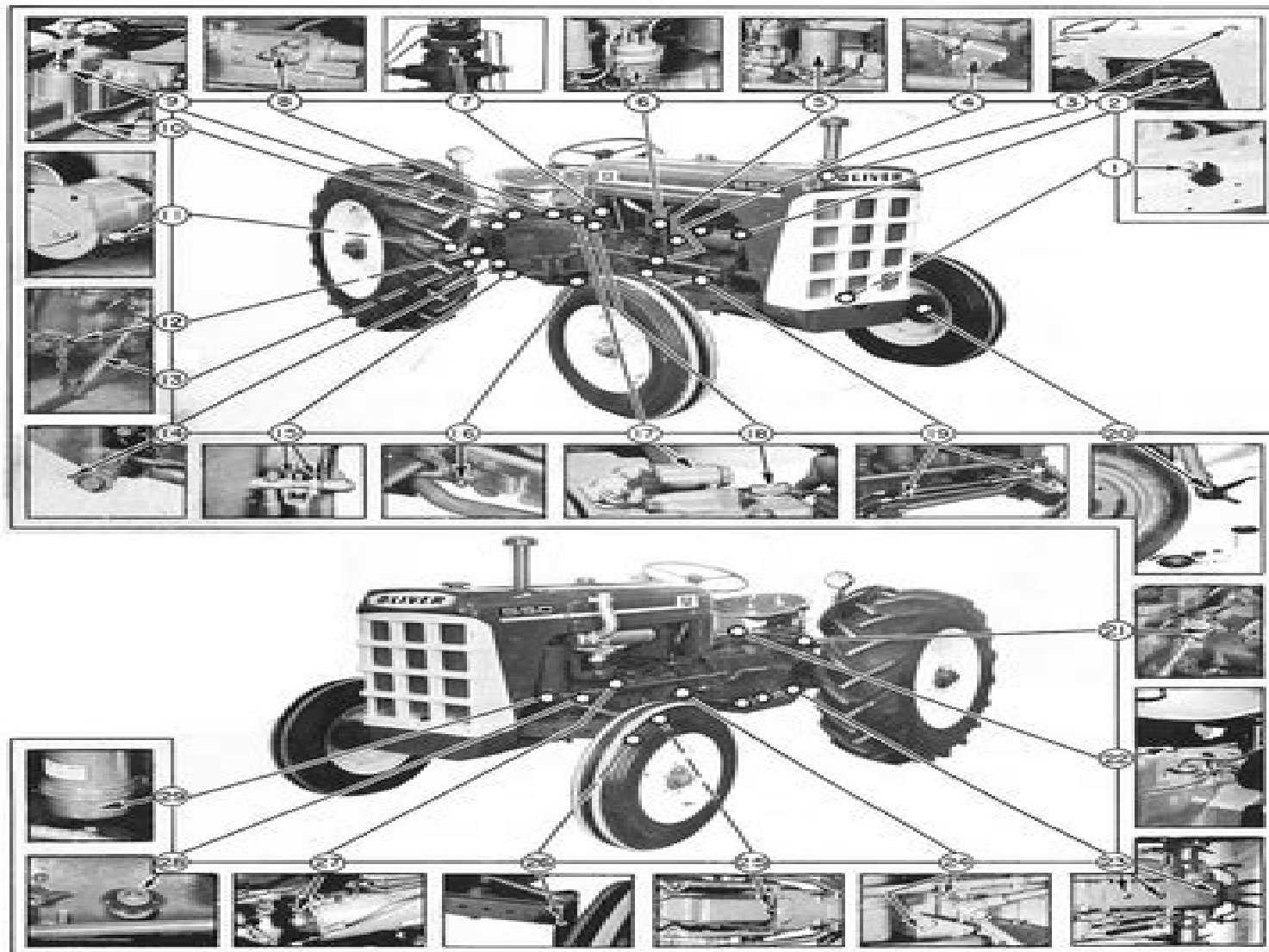
Figure 1-16 Lubrication Diagram
