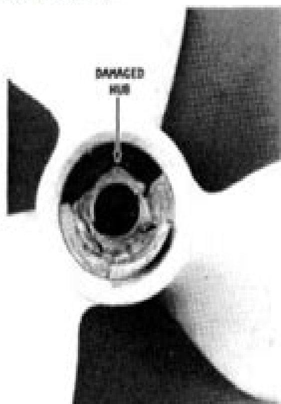
A cracked hub, caused by the propeller striking an underwater object. The rubber hub and propeller cleave may be replaced at nominal cost.
