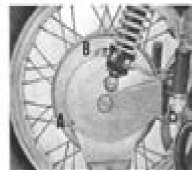
Rear wheel drive oil level, filler, and drain plugs (V750 and V750i)
