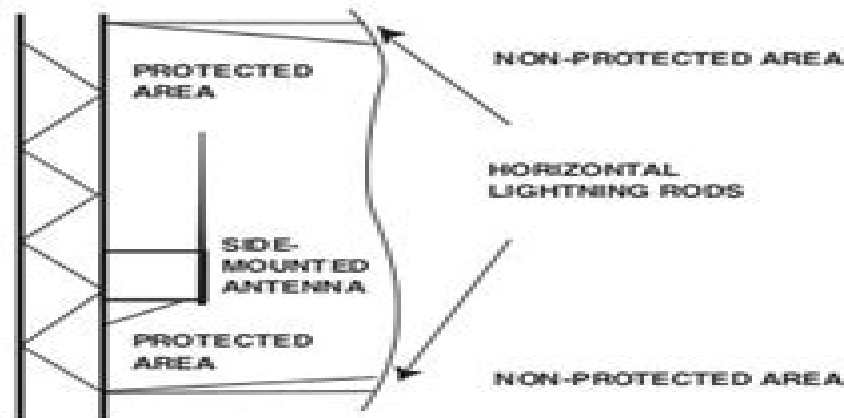
FIGURE 2-2 USING HORIZONTAL LIGHTNING RODS TO PROTECT SIDE-MOUNTED ANTENNA
