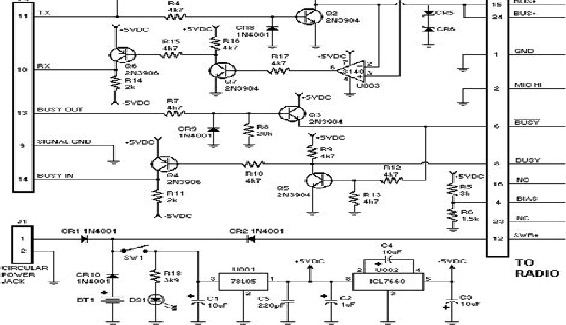
RADIO INTERFACE BOARD SCHEMATIC
