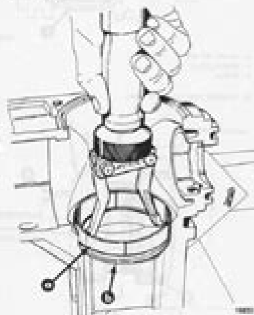
a - Bearing Cap b - Shaft
