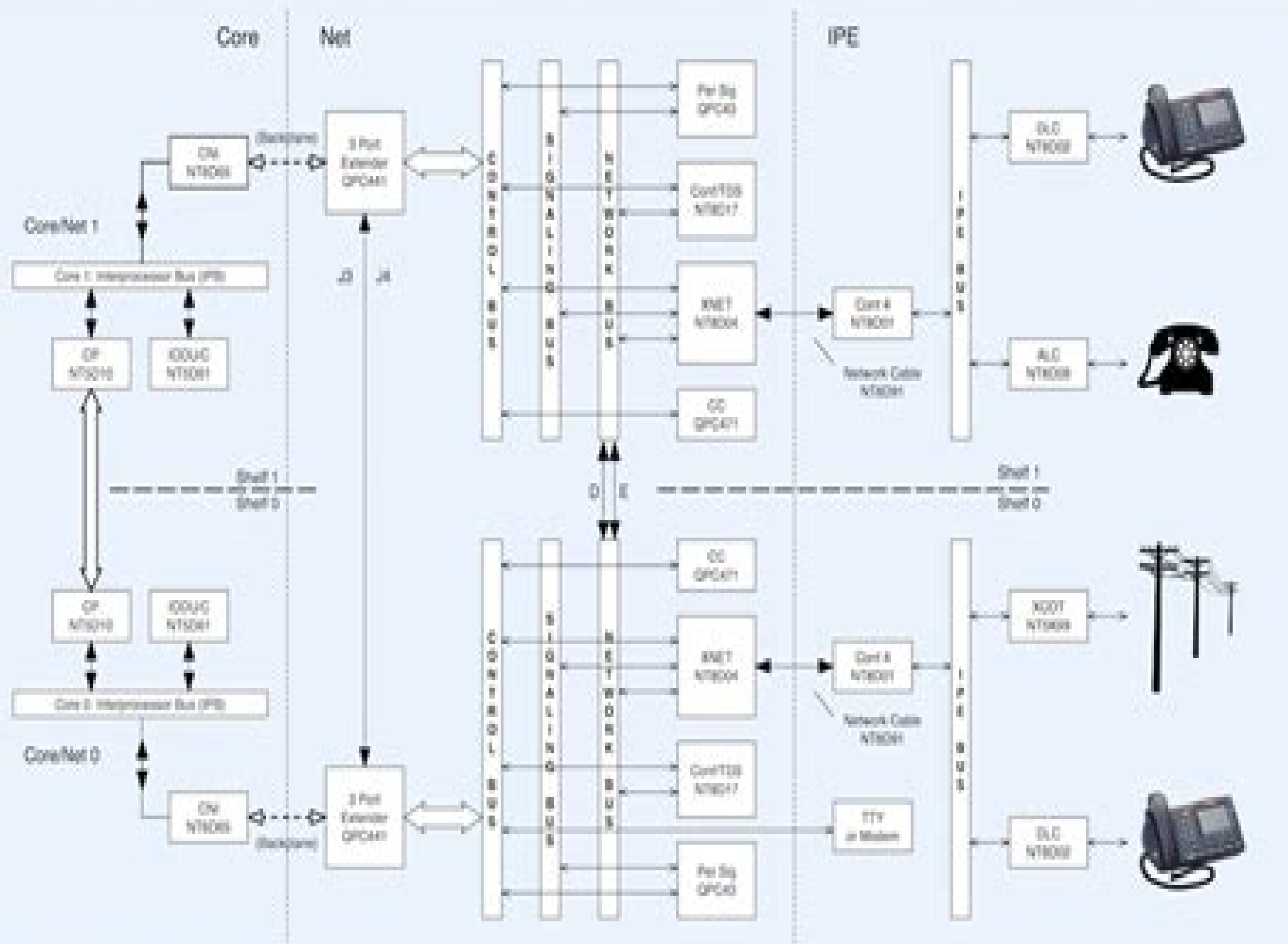
Option 61C Block Diagram
