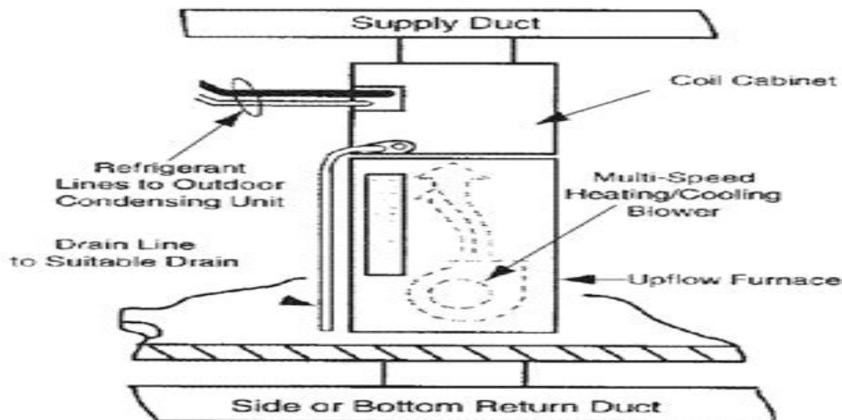
Figure 1. Upflow Furnace/Air Handler
