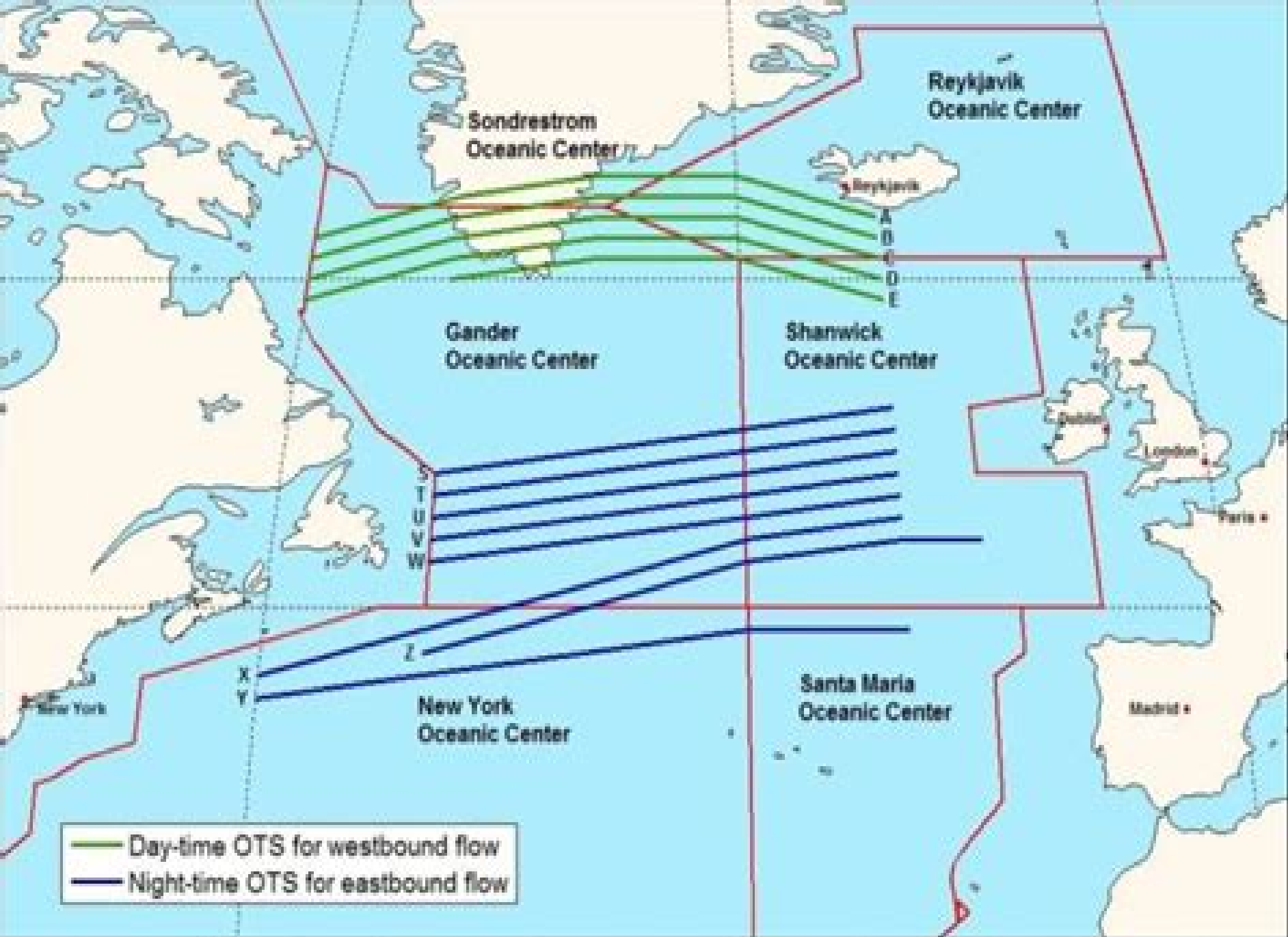
Figure 2: Illustration of NAT Oceanic Centers and the Track System (March 03, 2014)
