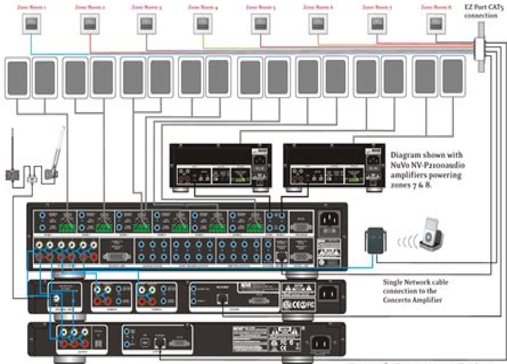
Grand Concerto Suite Wiring Diagram
