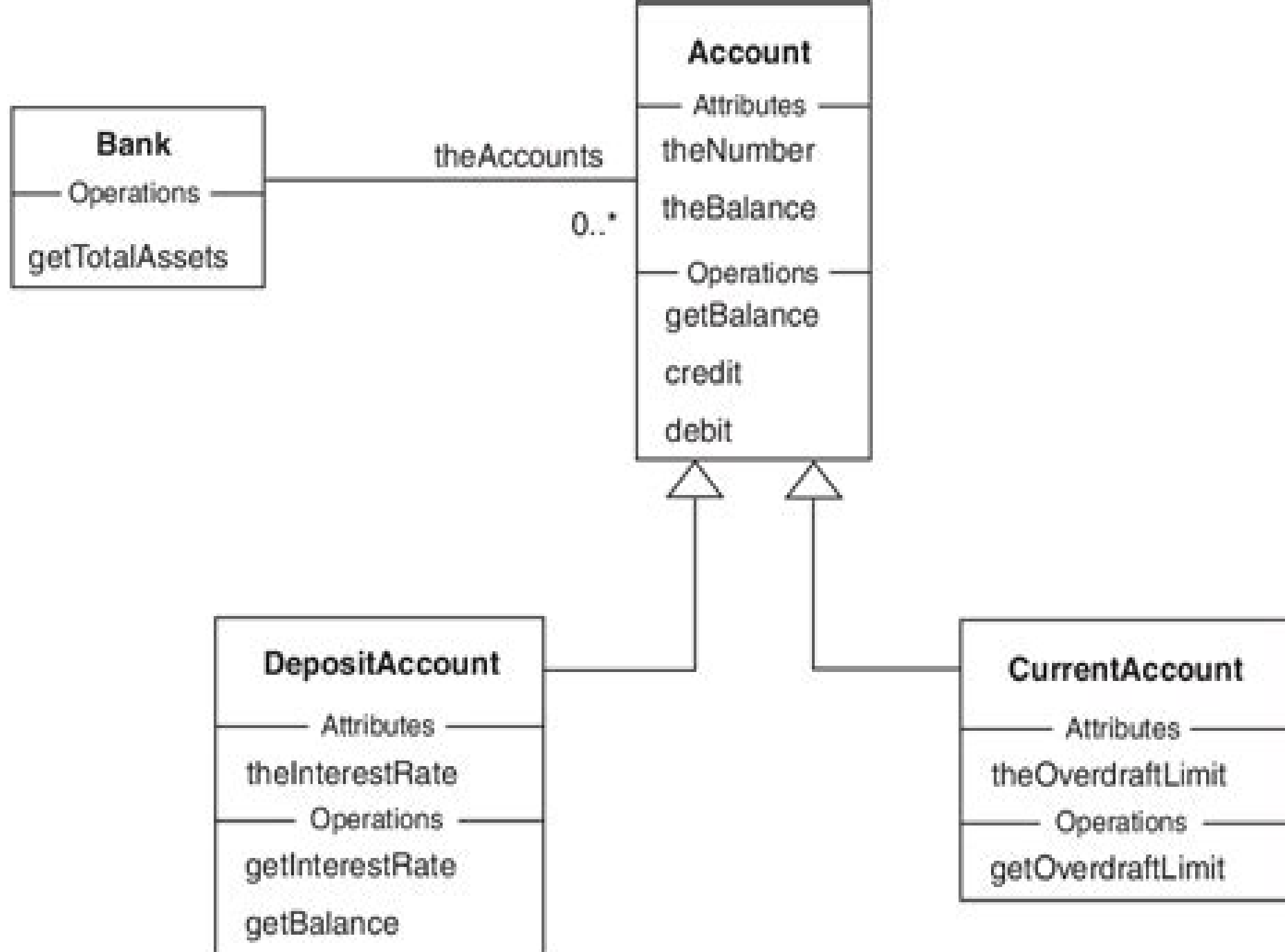
Figure 1.11: Bank/Account Class Diagram
