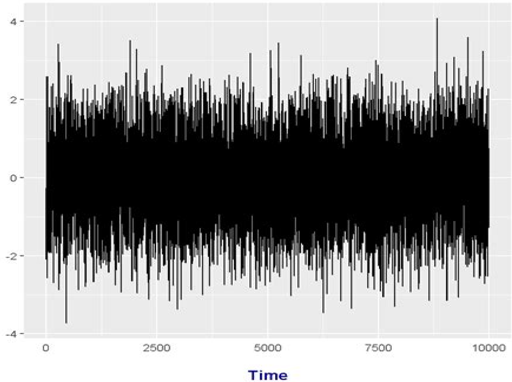
Simulated Observations From A White Noise Process
