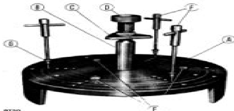
Component Parts of Ferodo Clutch Adjuster 291291/2
