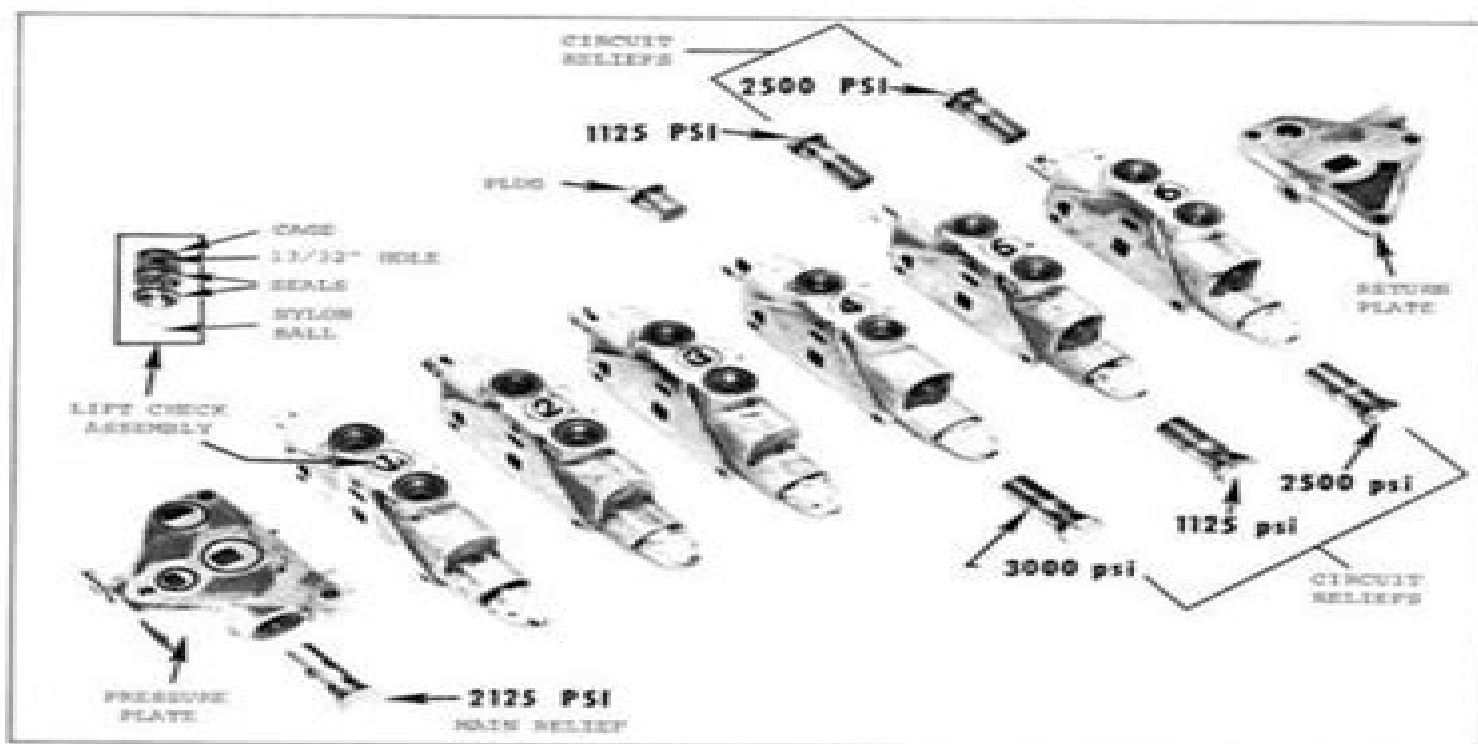
Fig. 11 - Identification of Valve "Working Sections" - NF Form No. 705-9-37 (4-62)
