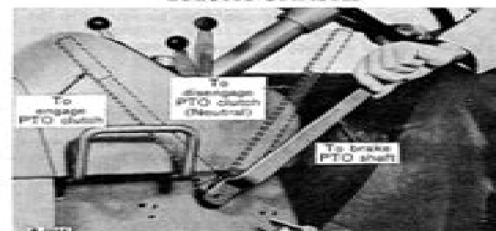
PTO Clutch Lever Operating Positions for John Deere 3010 and 4010 Series Tractors
