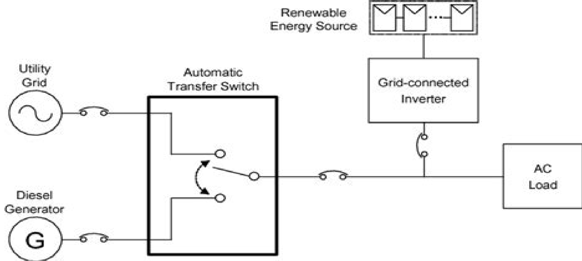
Fig. 1. Conventional power system with automatic transfer switch.
