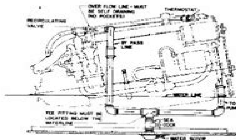
Fig. 4A—Piping Diagram for Engines with Dual Unit Thermostat. Pipe size for all external lines must never be smaller than the pump intake size
