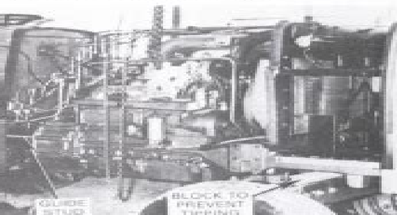
Fig. 197—View showing supports necessary when splitting. 3½" cylinder model is shown but blocking is similar for MF 1135.
