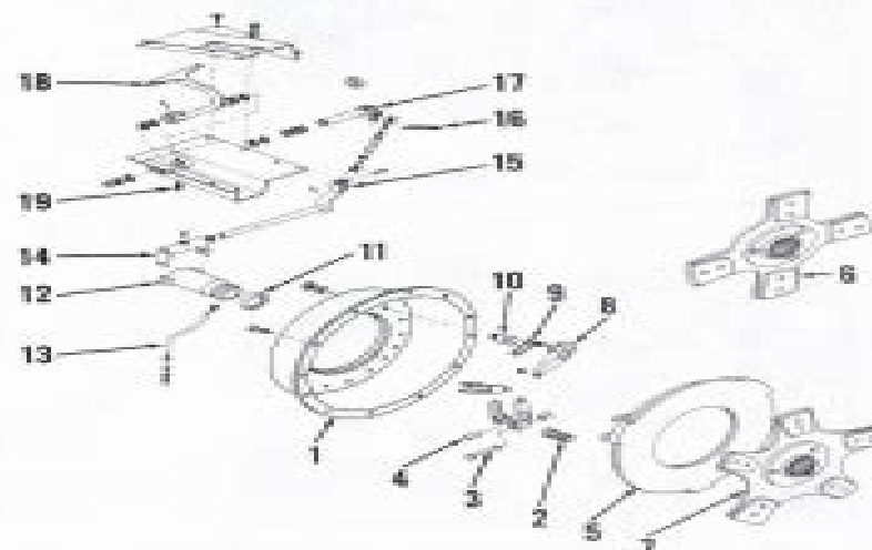
Fig. 198—Exploded view of clutch and linkage. Disc (6) with four pads is used with brown springs (2) on MF 1105 models only.
