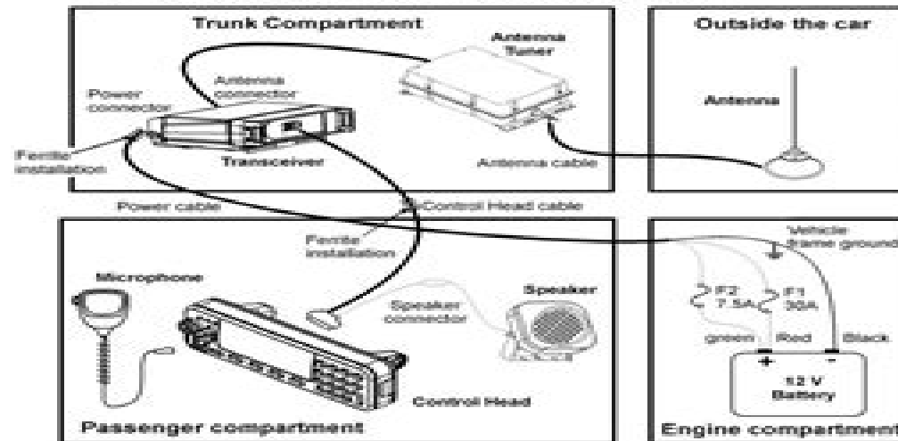
Figure 5: Trunk Model Installation Diagram
