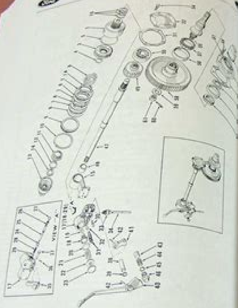
FIG. 100 - INDEPENDENT POWER TAKE OFF ASSEMBLY (1950 - 1955)
