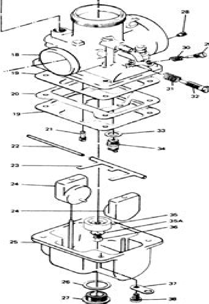
DIAGRAM A Exploded view of a SPIGOT MOUNT TYPE MIKUNI CARBURETOR
