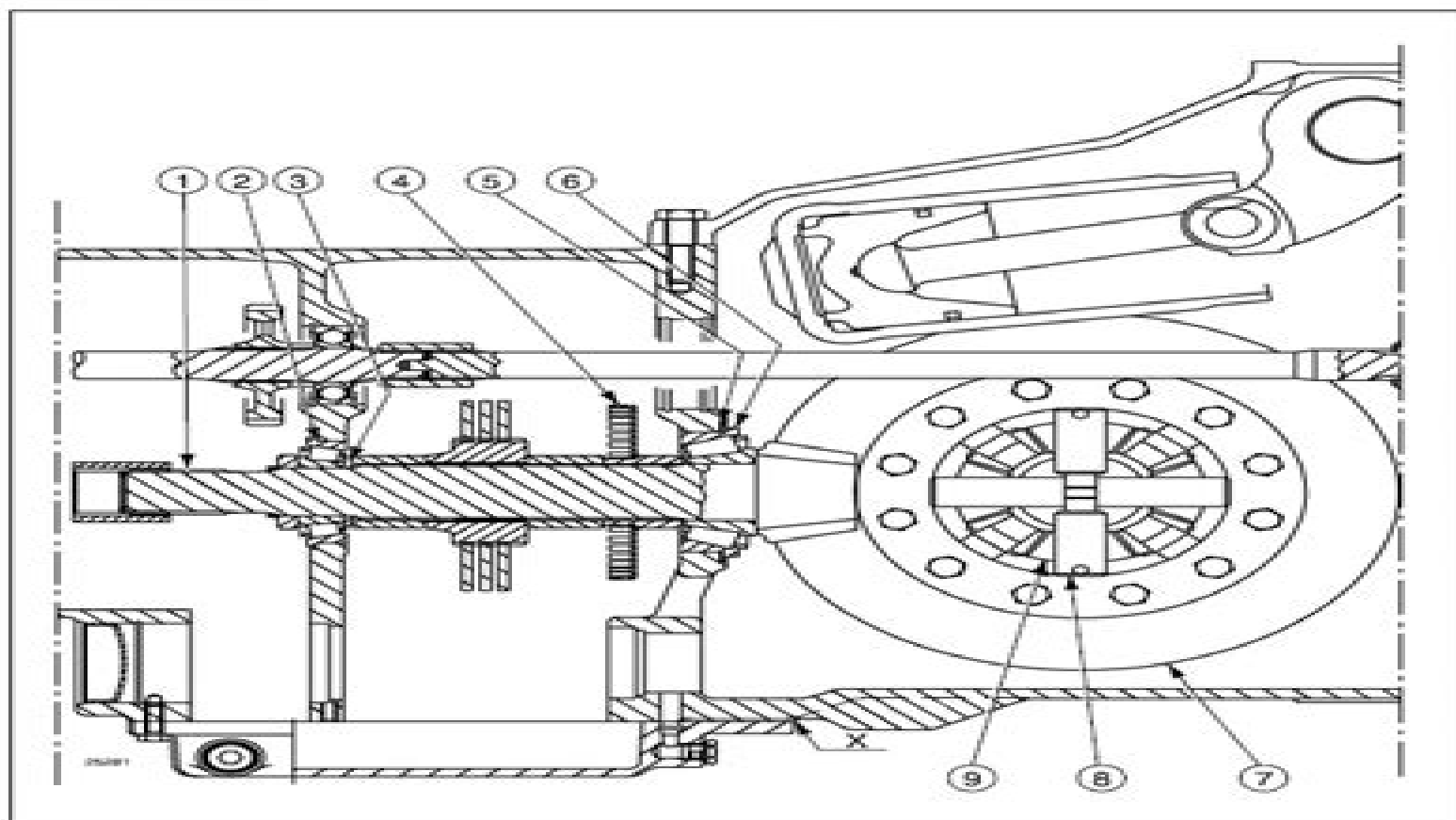
Rear Axle Longitudinal Sectional View
