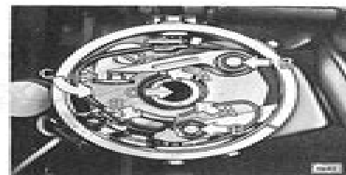
Figure 68-58 Lubricating Upper Distributor
