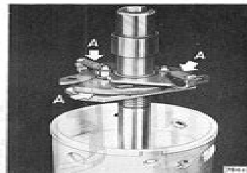
Figure 68-57 Lubricating Centrifugal Mechanism
