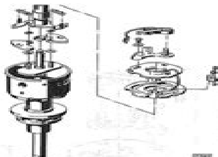
Figure 68-55 Removing Breaker Plate
