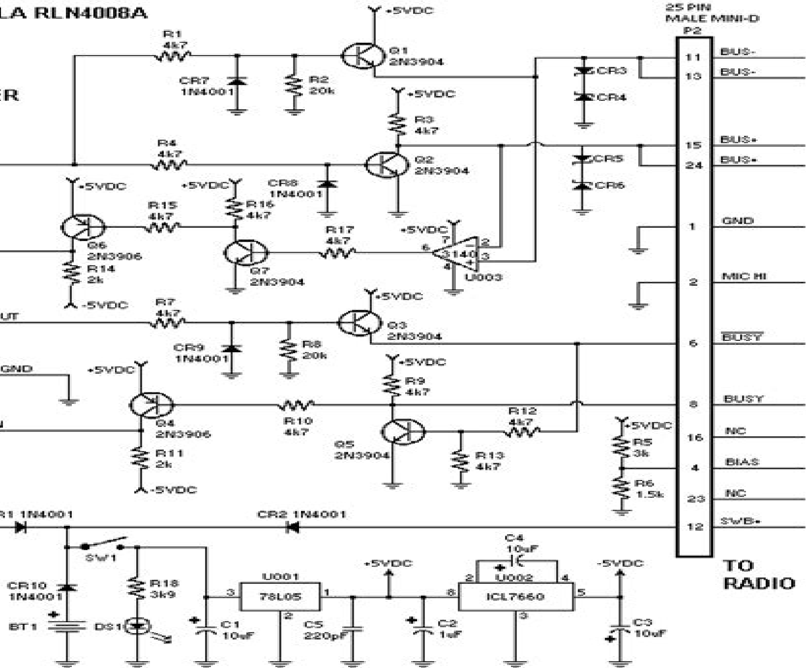
RADIO INTERFACE BOARD SCHEMATIC
