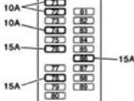
IPDM E/R fuse layout
