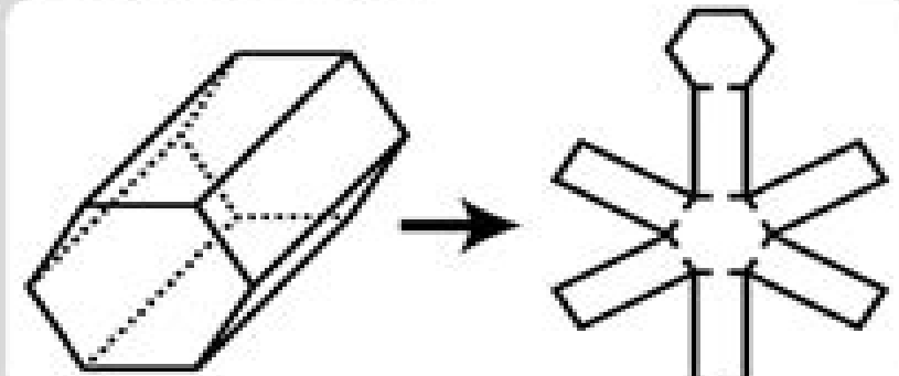
Hexagonal Prism
