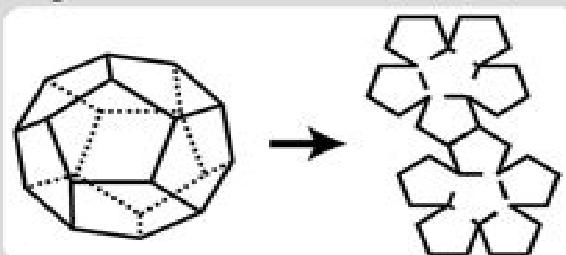
Regular Dodecahedron
