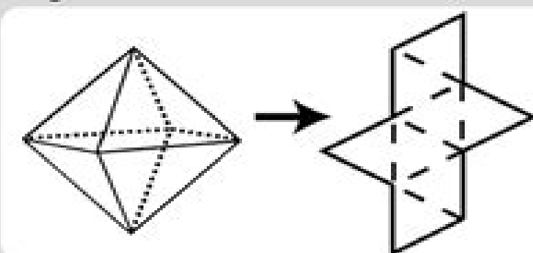
Regular Octahedron
