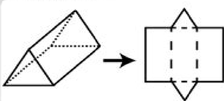
Triangular Prism
