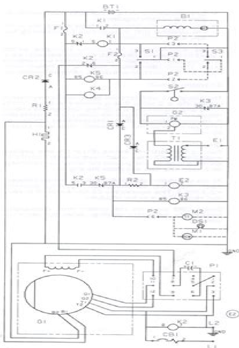
FIGURE 7-1. SCHEMATIC - 60 HERTZ
