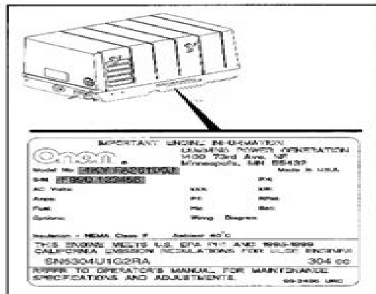
FIGURE 1-1. TYPICAL NAMEPLATE
