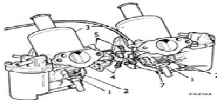
A twin-carburetter installation
