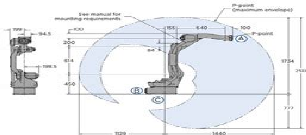
VIEW A
