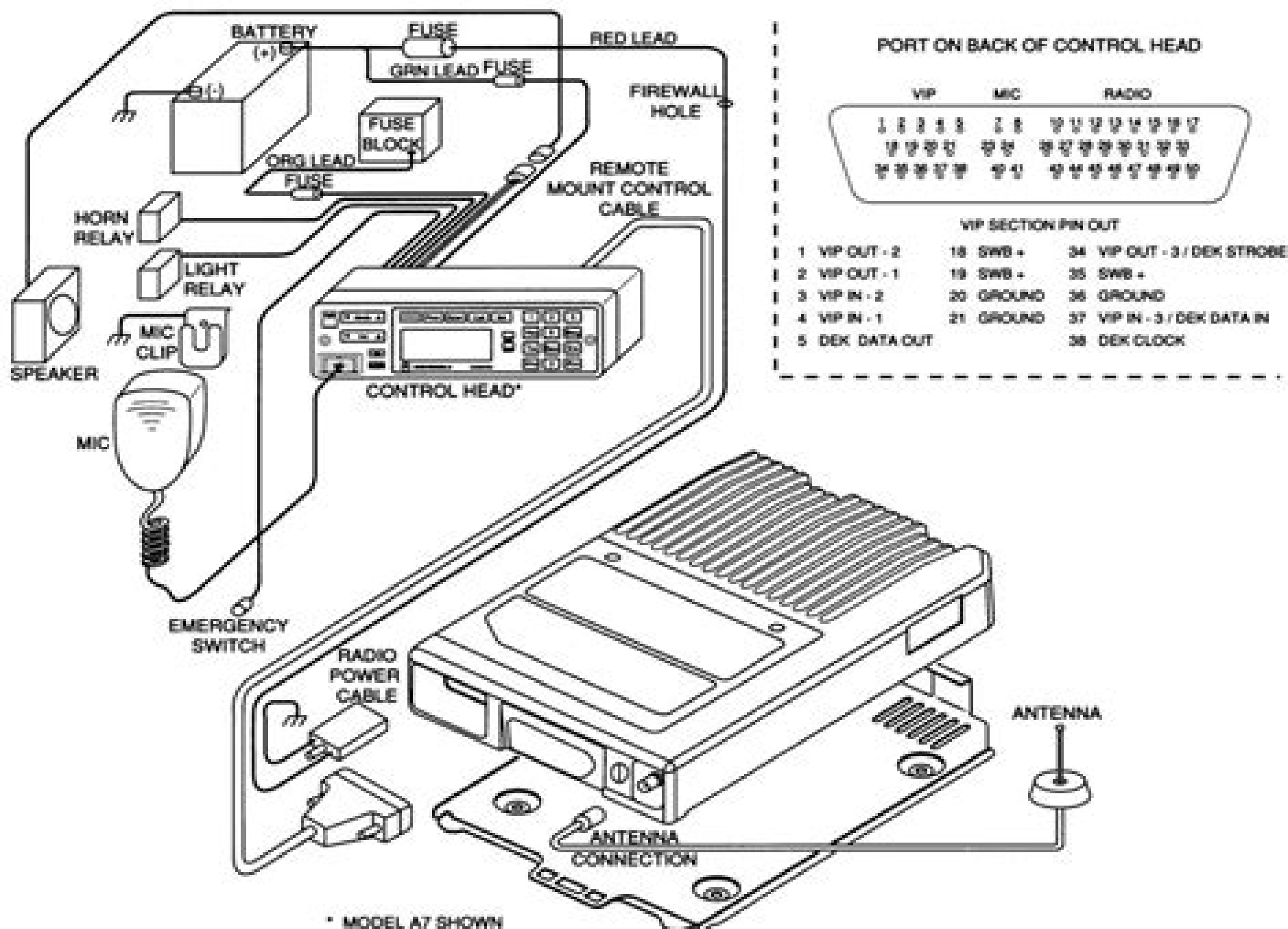
Figure 1. High-Power Radio Installation (Remote) Using A4, A5, A7 or A9 Control Heads
